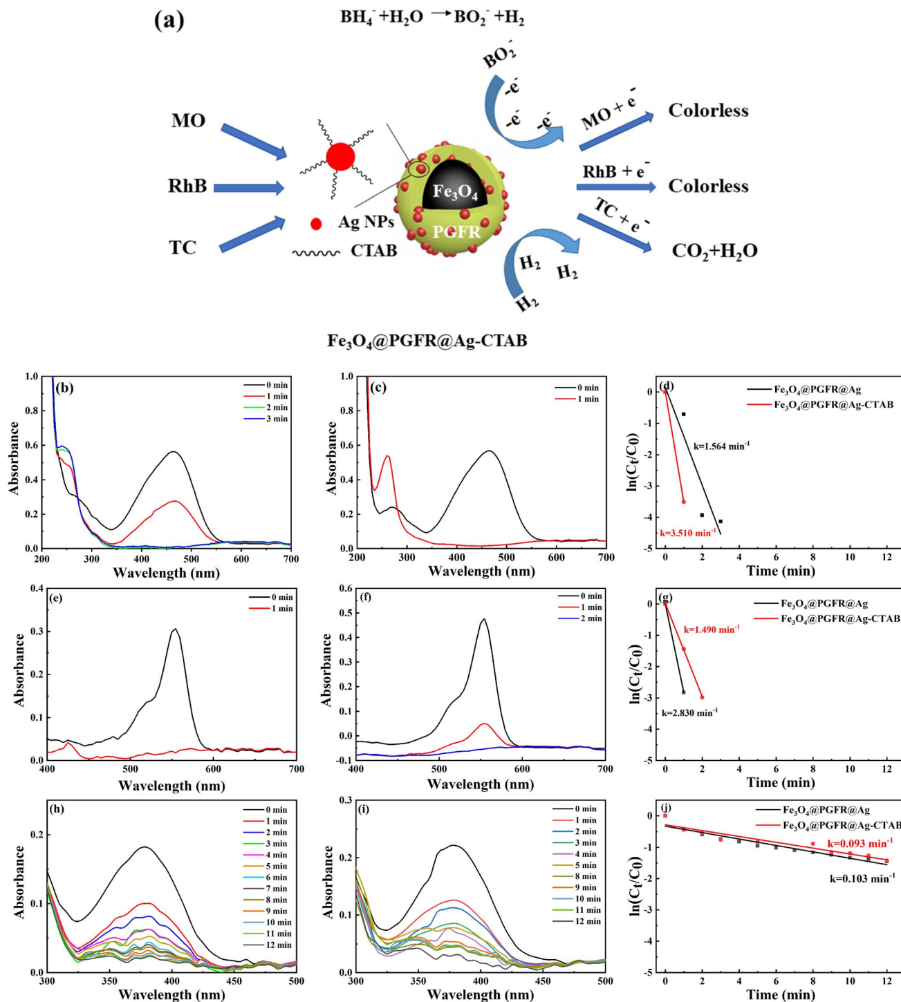
Fig. 10 (a) Schematic of the catalytic process. UV-vis spectra for MO: (b) \text{Fe}_3\text{O}_4@PGFR@Ag and (c) \text{Fe}_3\text{O}_4@PGFR@Ag-CTAB . (d) Comparison of first-order rates of reductive degradation. UV-vis spectra for RhB: (e) \text{Fe}_3\text{O}_4@PGFR@Ag and (f) \text{Fe}_3\text{O}_4@PGFR@Ag-CTAB . (g) Comparison of first-order rates of reductive degradation. UV-vis spectra for TC: (h) \text{Fe}_3\text{O}_4@PGFR@Ag and (i) \text{Fe}_3\text{O}_4@PGFR@Ag-CTAB . (j) Comparison of first-order rates of reductive degradation.
