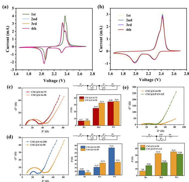
Fig. 8 (a) CV curves of CSC@S/Al cells with 50 μm thickness (b) CV curves of CSC@S/PAN-GF cells (c) different electrodes Nyquist curves and equivalent circuit parameters of electrodes (c) CSC@S/Al-50 and CSC@S/Al-75 (d) CSC@S/Al-50 and CSC@S/Al-250 (e) CSC@S/Al-50 and CSC@S/PAN-GF.
