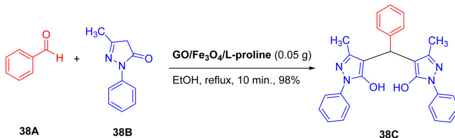
Scheme 38 Test reaction for investigation of catalytic activity of \text{GO/Fe}_3\text{O}_4/\text{L-pro} for the synthesis of bis-pyrazole under various conditions.
