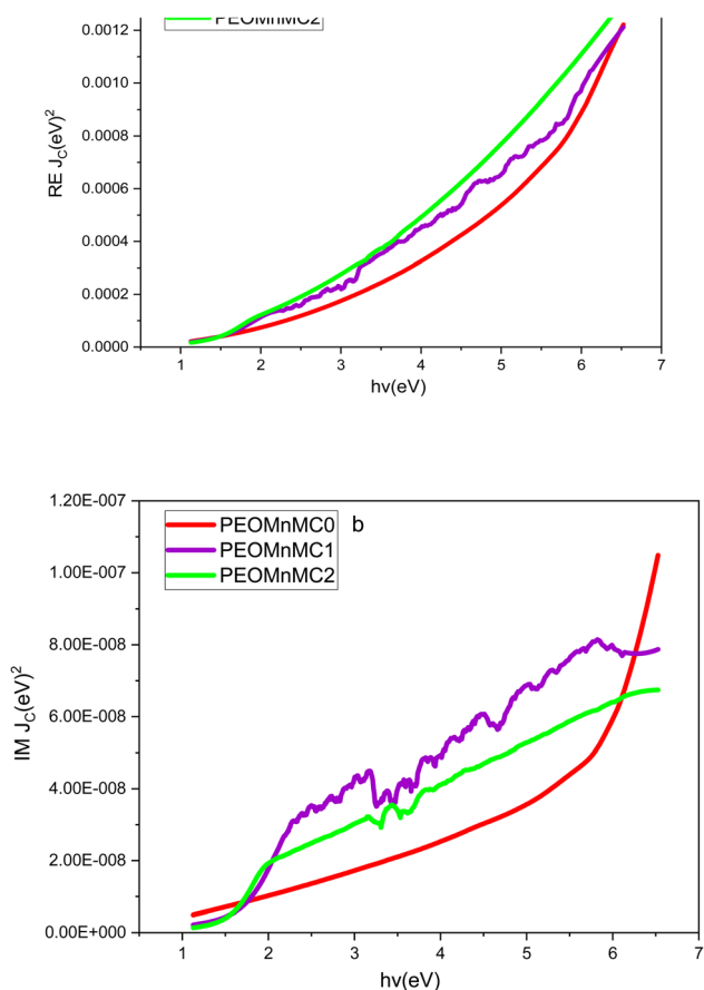
Fig. 13 (a and b) Plot (a) RE J_{CV} and (b) IM J_{CV} against of E_{\text{Photon}} Of for undoped and alter PEO polymer composites.
