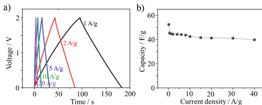
Fig. 23 Asymmetric capacitor of \text{MnO}_2 |1 M \text{Na}_2\text{SO}_4 aqueous electrolyte|ACM-CP-derived carbon: (a) charge/discharge curves at different current densities and (b) rate performance. 7 Reproduced from ref. 7 with permission from the Royal Society of Chemistry, copyright 2013.
