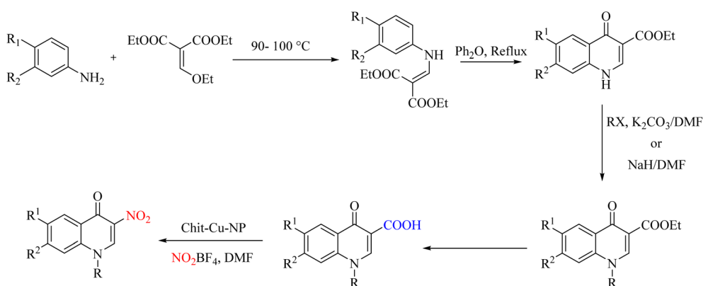
Scheme 28 Ipsso-nitration using polysaccharide-supported copper nanoparticles.
