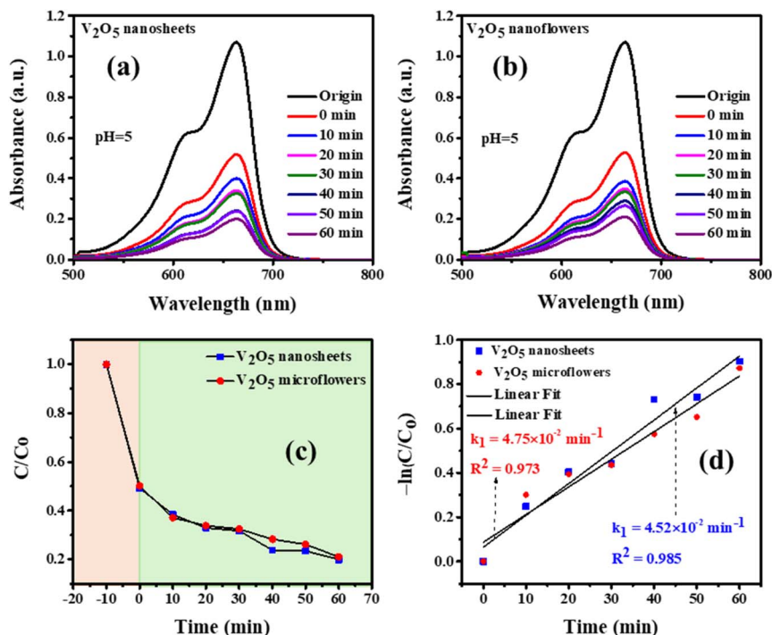
Fig. 8 Photocatalytic degradation of Methylene Blue (MB) under simulated sunlight using V 2 O 5 nanosheets and microflowers: (a) and (b) absorbance spectra over irradiation time, (c) photodegradation efficiency, and (d) ln(C/C 0 ) vs. irradiation time.
