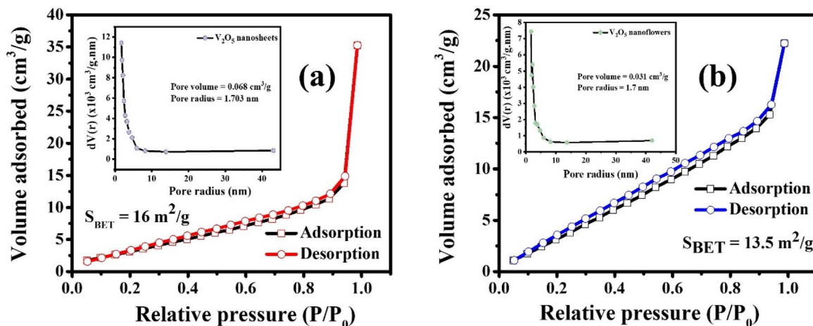
Fig. 6 Nitrogen adsorption/desorption isotherms of (a) nanosheet and (b) micro-flower samples annealed at 500^\circ\text{C} . Inset: pore size distribution of each nanomaterial.
