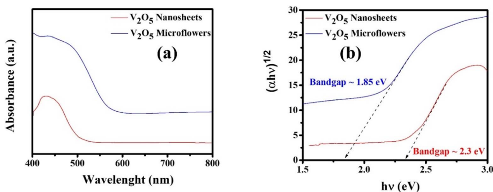
Fig. 7 UV-vis spectra of \text{V}_2\text{O}_5 nanosheets and microflowers samples (a), Tauc plots and estimated band gaps of the synthesized materials (b).
