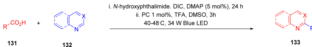
Fig. 63 Minisci reaction in the use of carboxylic acids in the presence of NAPs. 247
