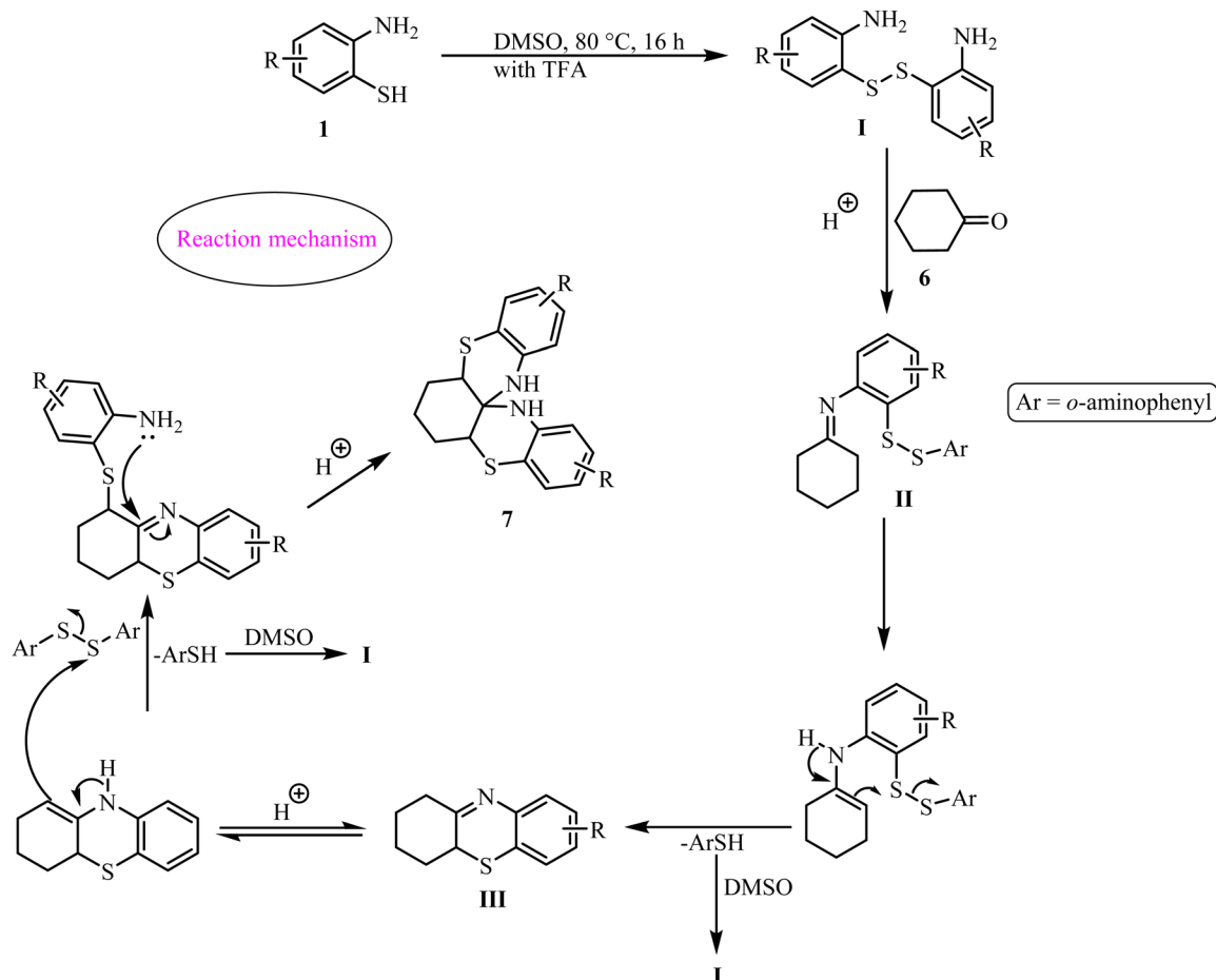
Scheme 3 Synthesis of 1,4-BT using 2-ATP and ketones.
