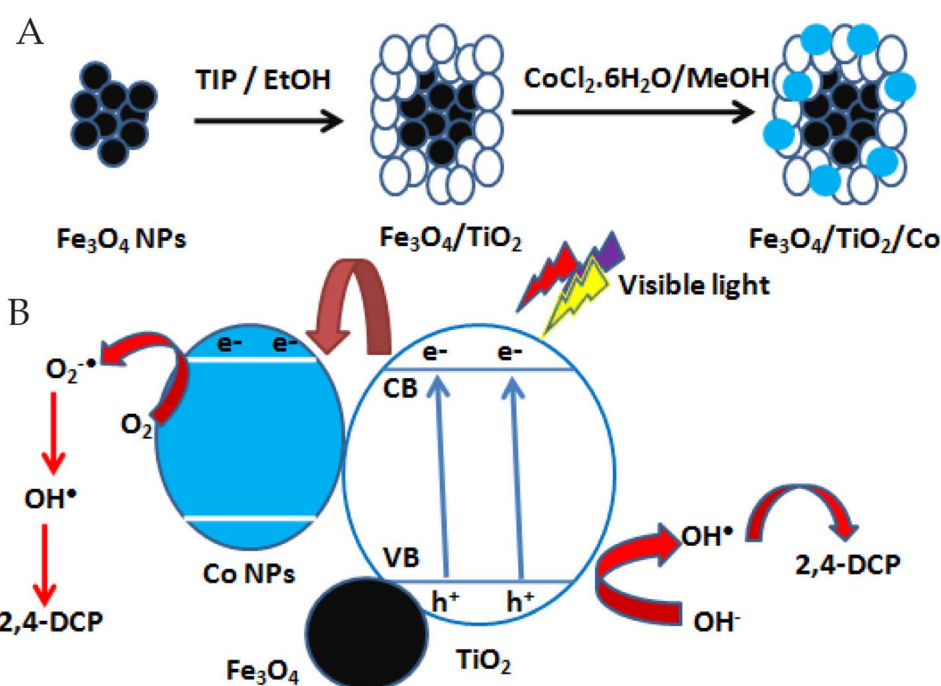
Fig. 4 2,4-Dichlorophenol degradation via photo-reactive \text{TiO}_2 nanoparticles, (A) preparation of the photocatalyst; (B) the degradation pathway of 2,4-DCP. 69
