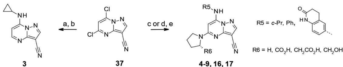
Scheme 30 Synthesis of acyclic pyrazolo[1,5- a ]pyrimidines. 154 a Reagents and conditions: (a) c -PrNH 2 , EtOH, 99%; (b) Pd/C, H 2 , EtOAc, 53%; (c) c -PrNH 2 or PhNH 2 or 6-amino-3,4-dihydroquinolin-2(1 H )-one, DIPEA, NMP, rt–100 °C, then pyrrolidine-R6, \mu w, 65–130 °C, 25–64%; (d) 6-amino-3,4-dihydroquinolin-2(1 H )-one, EtOH, 80 °C, 91%; (e) ( S ) or ( R )-prolinol, DIPEA, NMP, 80 °C, 65–67%. 154
