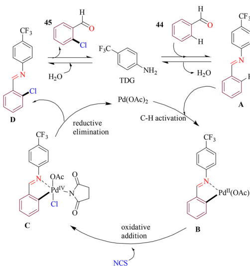
Scheme 20 Palladium-catalyzed ortho C–H chlorination of benzaldehydes.
