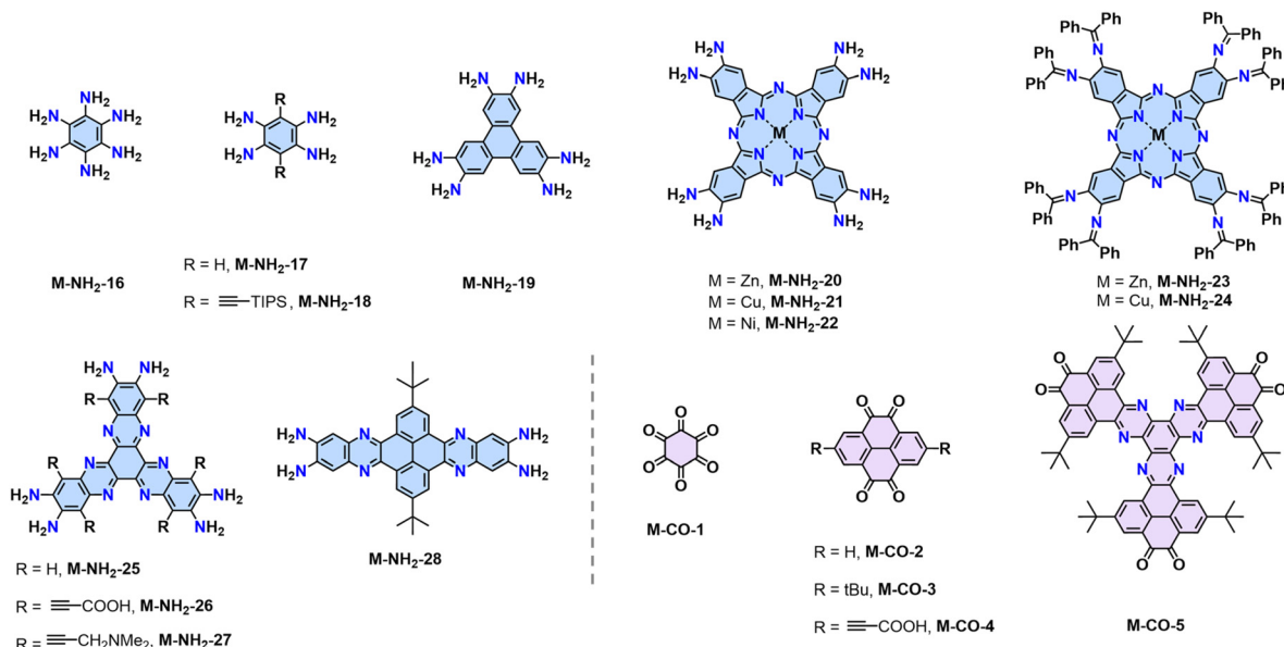
Fig. 4 Representative monomers contain multiple -\text{NH}_2 (blue) and -\text{C}=\text{O} (pink) groups at the -ortho positions to construct 2D PPZs.
