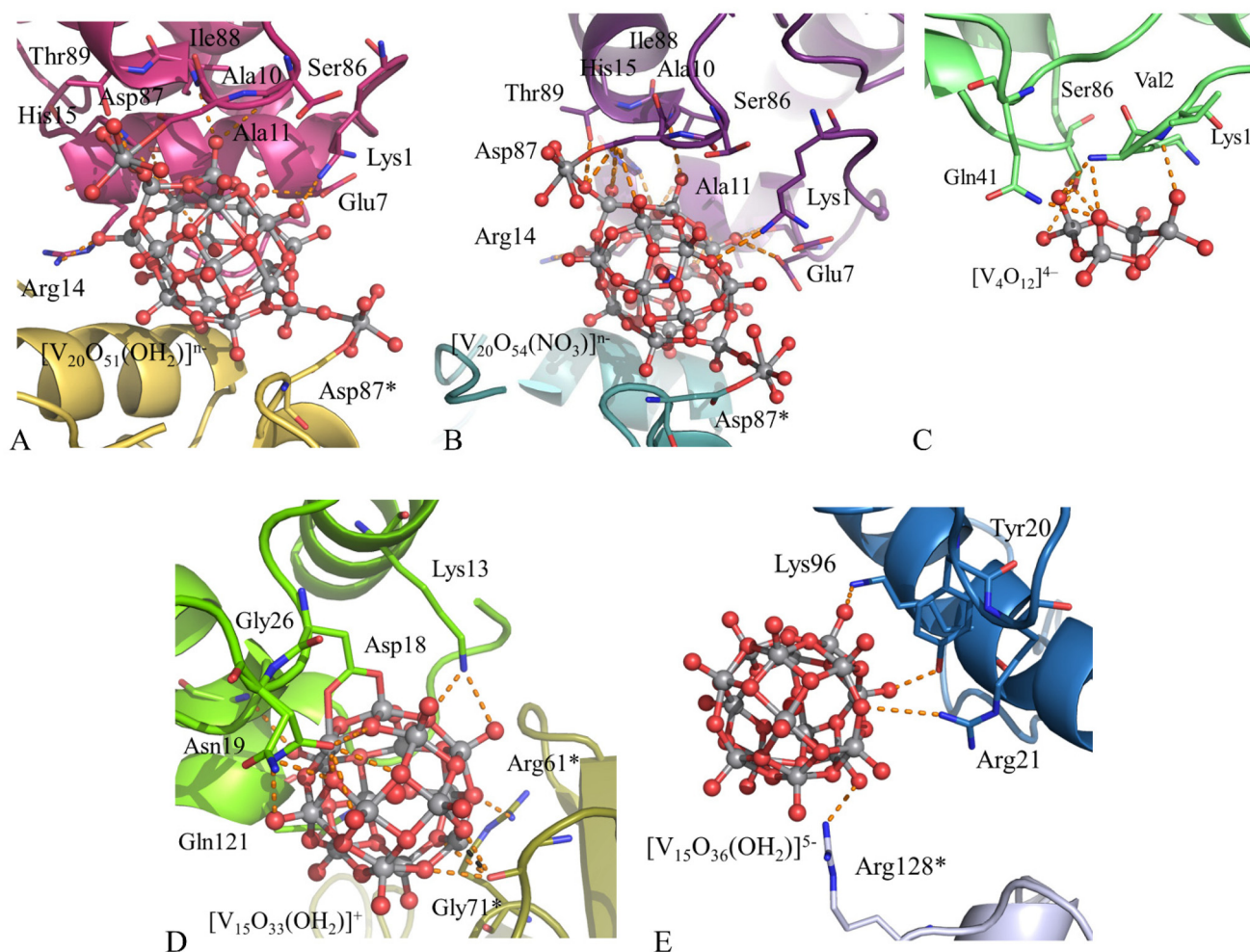
Fig. 10 Interactions of [V_{20}O_{51}(OH_2)]^{n-} (panel A), [V_{20}O_{54}(NO_3)]^{n-} (panel B), [V_4O_{12}]^{4-} (panel C), [V_7^V V_8^V O_{33}(OH_2)]^+ (panel D) and [V_7^V V_8^V O_{36}(OH_2)]^{5-} (panel E) with HEWL residues in crystals of the protein treated with [VO(acac)_2] .
