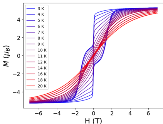
Fig. 4 Magnetic hysteresis measurements/hysteresis plot for 1 at a sweep rate of 20 mT s -1 .
