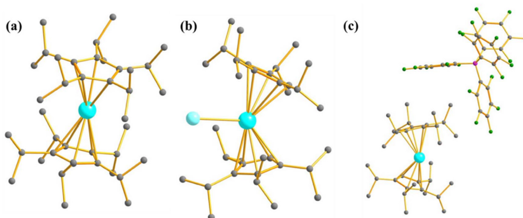
Fig. 15 The molecular structure of (a) [(\eta^5\text{-C}_5\text{Pr}_5)_2\text{U}]^+ ( 24 ) (b) [(\text{Cp}^t\text{Pr}_4)_2\text{U}] ( 25 ), and (c) [(\text{Cp}^t\text{Pr}_4)_2\text{U}][\text{B}(\text{C}_6\text{F}_5)_4] ( 26 ). Colour code: U (cyan), I (aqua), N (blue), Si (violet), B (pink), F (green), C (grey). Hydrogens are omitted for clarity.
