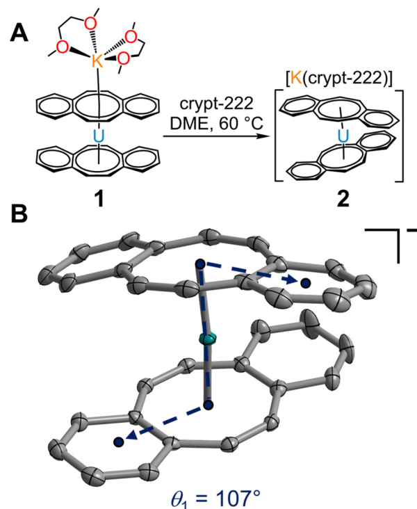
Fig. 3 (A) Synthetic route to [K(crypt-222)][U(dbCOT)_2] , 2 . (B) Structure of the [U(dbCOT)_2]^{2-} anion in a crystal of [K(crypt-222)][U(dbCOT)_2] , 2 , with thermal ellipsoids drawn at the 50% probability level. Teal and grey ellipsoids represent U and C atoms, respectively. H atoms and the [K(crypt-222)]^+ counteranion are omitted for clarity. Select interatomic distances (Å) and angles ( ^\circ ) for 2 : U–C COT = 2.690(3)–2.803(3); U–Cnt = 2.000, 2.003; Cnt–U–Cnt: 167.2. We define that the circles in each dbCOT drawing represent in total 18 \pi -electrons.
