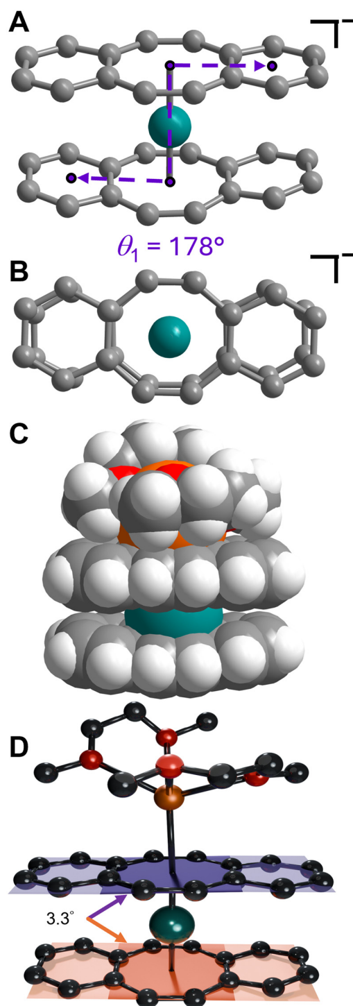
Fig. 2 (A) Structure of the [U(dbCOT)_2]^{2-} anion in a crystal of [K(DME)_2][U(dbCOT)_2] , 1 , with corresponding atom labels. The dihedral angles ( \theta_1 = 178^\circ and \theta_2 = 2^\circ ) were calculated using the benzo- and COT ring centroids. (B) Aerial perspective of 1 . Teal and grey spheres represent U and C atoms, respectively. H atoms and the coordinating [K(DME)_2]^+ counteranion are omitted for clarity. (C) Space filling model of 1 . Teal, orange, red, grey, and white-grey spheres represent U, K, O, C, and H atoms, respectively. (D) Structure of 1 with planes bisecting the central COT rings of each dbCOT^{2-} ligand, where the angle between planes is 3.3^\circ . Teal, orange, red, and black spheres represent U, K, O, and C atoms, respectively. H atoms are omitted for clarity.
