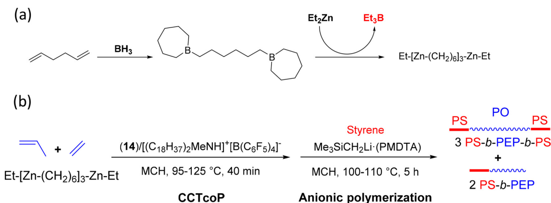
Scheme 47 (a) Synthesis of the dialkylzinc species. (b) Preparation of PS-b-PEP-b-PS triblock copolymers by switching from E/P CCTcoP to anionic polymerization of styrene by using \text{Me}_3\text{SiCH}_2\text{Li(PMDTA)} as a preinitiator. 71
