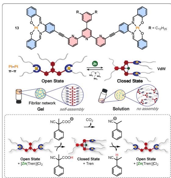
Fig. 12 Structure of \text{terpy}(\text{Pt-Salphen})_2 -based tweezers 13 and schematic representation of sol-gel transitions through the mechanical switching of the molecular tweezers. Inlay of transient disassembly and reassembly controlled by the chemical fuel 2-cyano-2-phenylpropanoic acid in a multicomponent system composed of tweezers 13 and [\text{Zn}(\text{Tren})]\text{Cl}_2 in toluene. Reproduced from ref. 21 with permission from American Chemical Society, copyright 2025.
