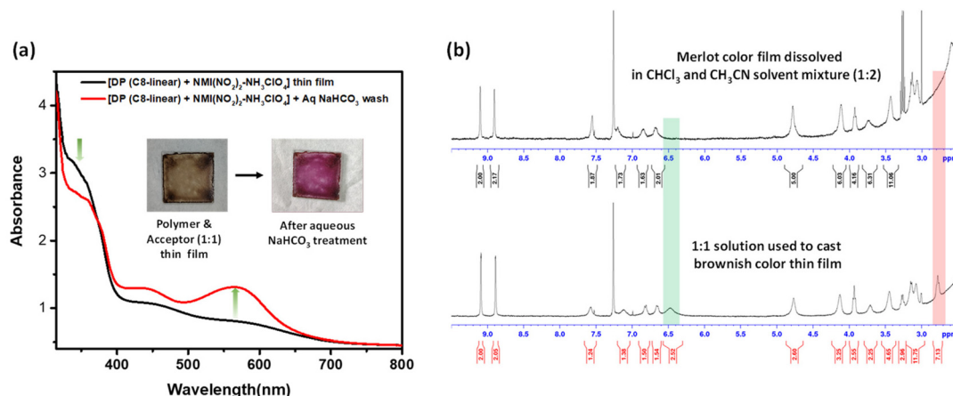
Fig. 5 (a) UV-visible spectra of the thin film cast on quartz plates, before (black) and after (red) treatment with aqueous \text{NaHCO}_3 solution. (b) ^1\text{H-NMR} spectra of the solution obtained by dissolving the films in \text{CDCl}_3 and \text{CH}_3\text{CN} (1 : 2), before and after \text{NaHCO}_3 treatment.
