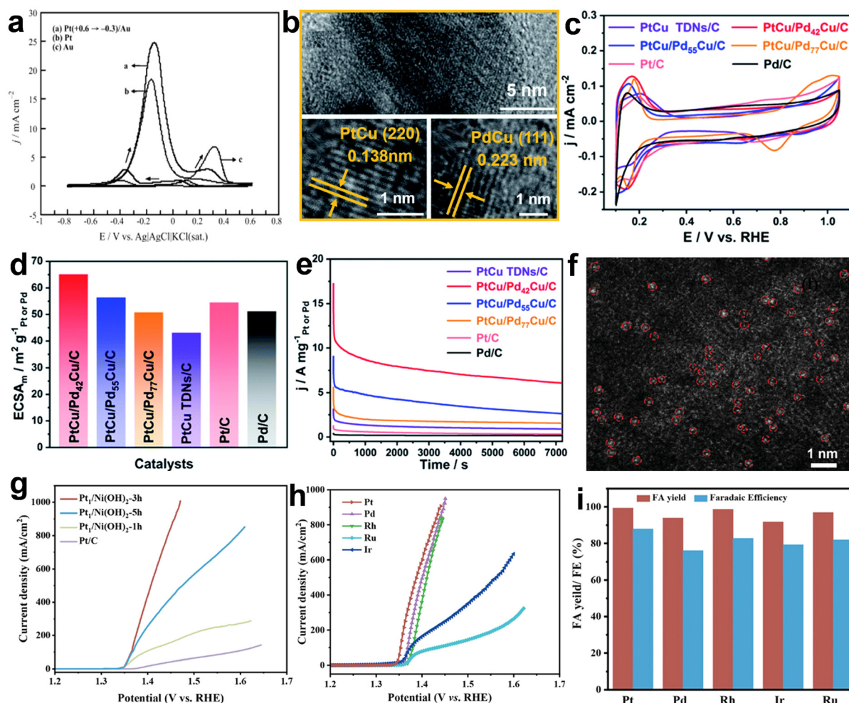
Fig. 11 (a) CV of Pt (+0.6 \rightarrow -0.3)/Au, Pt and Au electrodes in 0.6 M NaOH with 0.1 M glycol at a scanning rate of 60 mV s -1 , reproduced with permission. 63 Copyright 2010, Elsevier. (b) HRTEM images of PtCu/Pd 77 Cu core-shell TDNs, (c) CV curves of different catalysts at 60 mV s -1 scanning rate in the electrolyte, (d) ECSA histogram of different catalysts, (e) i - t curves of different catalysts in electrolyte solution at 1.0 M KOH with 1.0 M EG, reproduced with permission. 64 Copyright 2022, American Chemical Society. (f) HAADF-STEM images of Pt/Ni(OH) 2 -3 electrocatalysts, (g) EGOR properties of different samples, (h) and (i) properties of other elements, reproduced with permission. 65 Copyright 2024, John Wiley and Sons.
