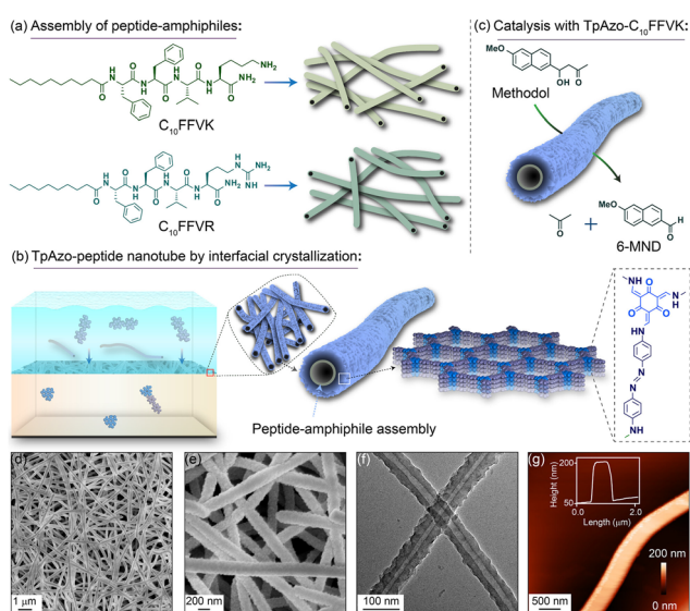
Fig. 15 Diagrammatic representation of the process: (a) self-assembly of C 10 FFVK and C 10 FFVR peptides into nanotubes, (b) synthesis of TpAzo-peptide nanotubes via interfacial crystallization, and (c) catalysis with TpAzo–C 10 FFVK nanotubes. (d) and (e) SEM images, (f) TEM image, and (g) AFM image of TpAzo–C 10 FFVK nanotubes. Adapted with permission from ref. 175. Copyright 2023 American Chemical Society.
