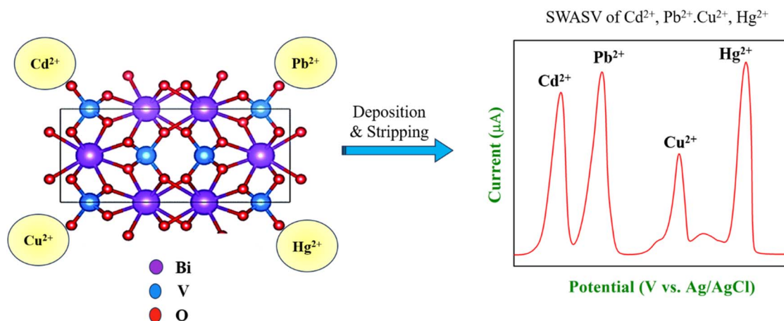
Fig. 8 The graphical illustration of the adsorption mechanism of heavy metal ions on the surface of BiVO 4 /GCE in 0.1 M HEPES buffer determined by SWASV. 50
