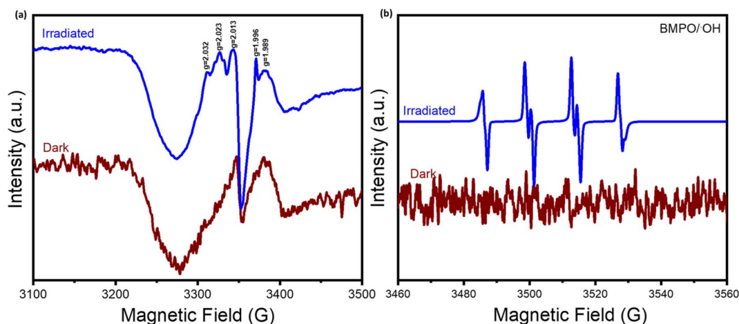
Fig. 8 (a) EPR spectra of the Au SA/TiO 2 sample under subsequential dark and light conditions at 90 K. (b) The spin trapping tests of Au SA/TiO 2 for detecting hydroxyl (·OH) radical formation by using 5- tert -butoxycarbonyl-5-methyl-1-pyrroline- N -oxide (BMPO) as a spin trapping agent.
