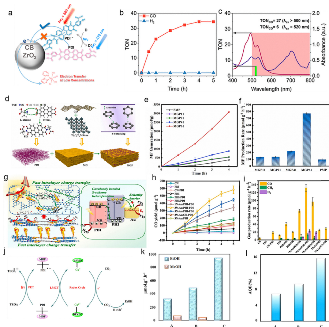
Fig. 16 (a) Strategy for photogeneration of a potent and long-lived \text{ZrO}_2(\text{e}^-) . (b) TON of CO and \text{H}_2 by \text{Re}(\text{bpy})(\text{CO})_3\text{Cl} and \text{ZrO}_2|\text{PDI} as a function of irradiation time. (c) Photocatalytic \text{CO}_2 reduction TON under 520 nm irradiation or broad band irradiation with wavelengths greater than 500 nm. Reproduced from ref. 141. Copyright 2022, American Chemical Society. (d) Schematic illustration of the MXene/GO/PDI composite aerogels. (e) MF generation yield of samples changing over time under the irradiation for 4 h. (f) MF generation rate of samples under the irradiation for 4 h. Reproduced from ref. 142. Copyright 2022, Elsevier. (g) Proposed photocatalytic mechanism for Au/PHI-PDI. (h) Time-dependent CO evolution performances. (i) Stability test over the 3%Au/PHI-PDI. Reproduced from ref. 143. Copyright 2025, Elsevier. (j) Proposed photocatalytic mechanism for Cu@PDI(30%)-NZU67. (k) Photocatalytic activity: Cu@PDI(30%)-NZU67 (50 mg), irradiation wavenumber = 420 nm, TEOA (0.3 M), and MeCN/deionized \text{H}_2\text{O} (4 : 1 v/v). (l) AQE results of Cu@PDI(30%)-NZU67. Reproduced from ref. 147. Copyright 2024, Elsevier.
