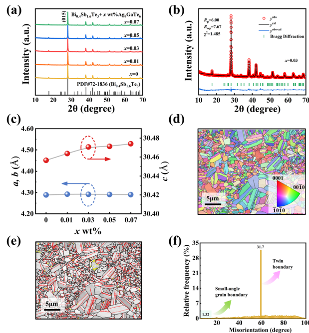
Fig. 1 Microstructure changes induced by \text{Ag}_9\text{GaTe}_6 doping. (a) The XRD patterns of \text{Bi}_{0.4}\text{Sb}_{1.6}\text{Te}_3 + x \text{ wt\% Ag}_9\text{GaTe}_6 , Rietveld refined XRD patterns of (b) x = 0.03 at room temperature. (c) Variation of the lattice constants. (d) The inverse pole-figure mapping of the EBSD image for x = 0.03 sample. (e) Kikuchi band contrast map and (f) grain boundary misorientation distribution of x = 0.03 sample.
