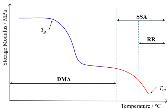
Fig. 2 Test ranges of dynamic mechanical analysis (DMA), rotational rheometry (RR) and successive self-nucleation and annealing (SSA) protocol.
