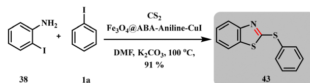
Scheme 19 \text{Fe}_3\text{O}_4@ABA -aniline- \text{CuI} catalysed synthesis of 2-(phenylthio)benzothiazole (Sun et al. ).
