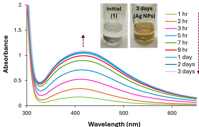
Fig. 19 Electronic spectral changes as a function of time during the formation of silver NPs by the IMR reaction of the Ag I complex ( 1 ) in methanolic solution (417 \mu M).
