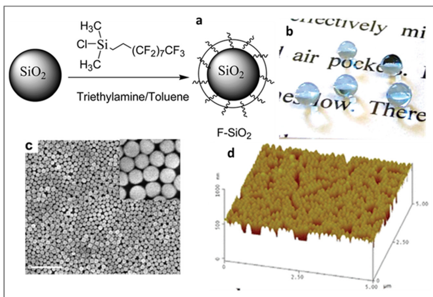
Fig. 10 (a) Schematic illustration of the synthesis of fluorosilane-coated silica nanoparticles, (b) optical photographs of water droplet-coated poly-ester fabric, and (c) surface morphology from SEM and (d) AFM images. Reproduced with permission from ref. 59, ACS, Copyright 2012.
