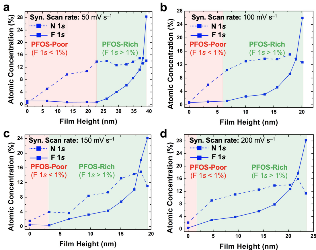
Fig. 4 Representative elemental analyses using XPS SDP for MIP films imprinted with PFOS using different synthesis scan rates ("syn. scan rate"): (a) 50, (b) 100, (c) 150, and (d) 200 mV s -1 . We used the N 1s signal to designate the presence of the MIP films and the F 1s signal for the presence of imprinted PFOS. We defined the PFOS-poor region where the F 1s signal was less than 1% of the atomic concentration, and the PFOS-rich region where the F 1s signal was greater than 1%.
