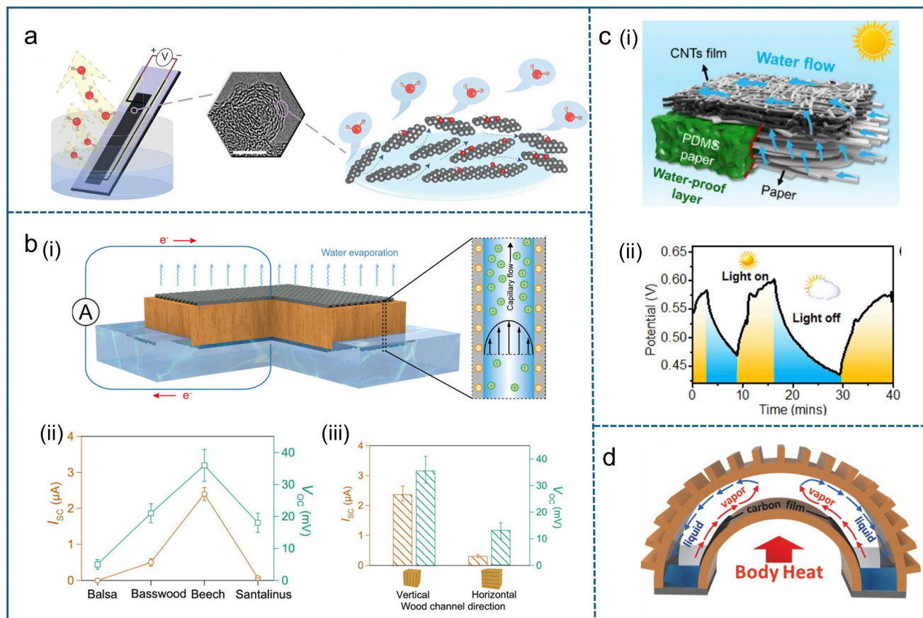
Fig. 24 Applications of an evaporation energy generator. a ) Schematic of the setup for harvesting energy from water evaporation through CB film. Reproduced with permission. 353 Copyright 2017, Springer Nature. b ) (i) Schematic of the electricity generation induced by evaporation in a piece of wood. The microchannels of the wood piece are vertically aligned. When water flows in the microchannels, the inner surfaces of the channel are negatively charged, resulting in a positively charged flow. b ) (ii) and (iii) Output voltage and current of different wood species and wood channel direction. Reproduced with permission. 364 Copyright 2020, American Chemical Society. c ) (i) Schematic of the solar-driven evaporator using a bilayer carbon nanotube/cellulose paper structure. c ) (ii) Under solar irradiation, the electrical output was enhanced compared to the dark environment. Reproduced with permission. 372 Copyright 2020, Elsevier. d ) Schematic of the self-powered wearable wristband. While DI water evaporated, driven by body heat, the porous carbon membrane harvested the energy from evaporation to electricity. Reproduced with permission. 374 Copyright 2018, Wiley.
