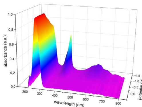
Fig. 2 Spectroelectrochemical measurements of MVCl_2 illustrating the appearance of MV^{•+} in TFE.
