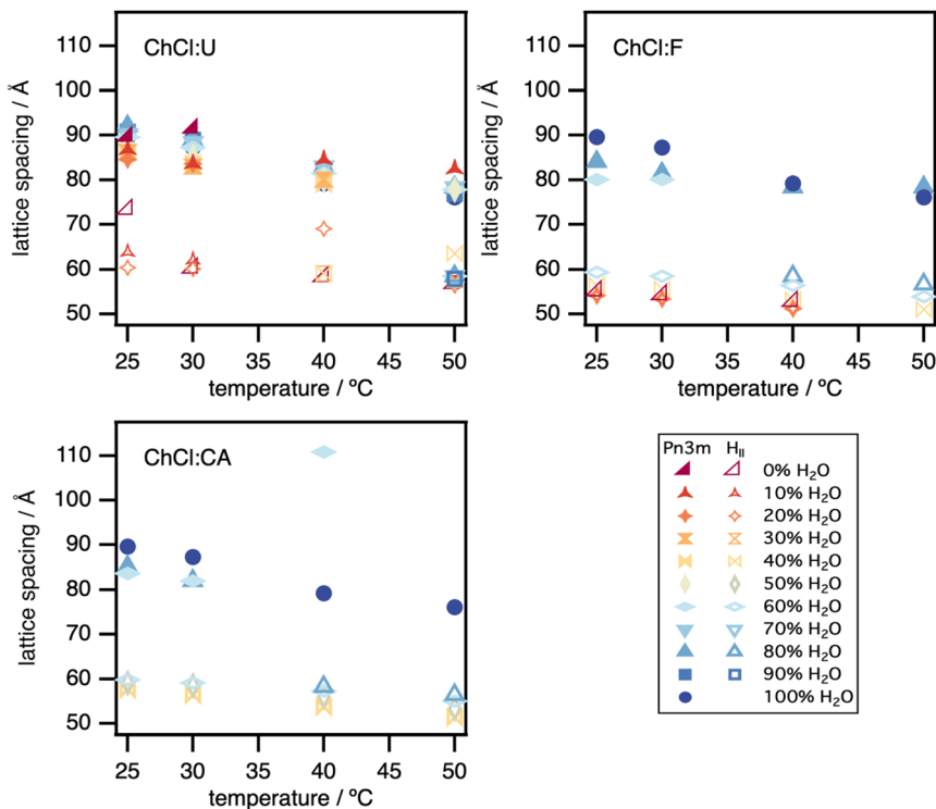
Fig. 7 Lattice spacings for the Pn3m cubic and H_{II} phases observed for monoolein in ChCl: U-water, ChCl: F-water and ChCl: CA-water mixtures. The error bars are smaller than the marker sizes. Where two H_{II} phases are observed, the larger lattice spacing is plotted.
