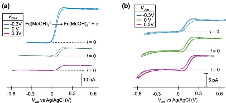
Fig. 3 Cyclic voltammograms of 2 mM ferrocenedimethanol ( \text{Fc}(\text{MeOH})_2 ) at (a) pH = 7 and (b) pH = 1 at V_{\text{bias}} = -0.3, 0 , and 0.3 V. Each condition shows 2 cycles of voltammetry.
