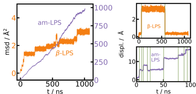
Fig. 2 MSD for \beta -LPS and am-LPS using the UFP. MSD of am-LPS and \beta -LPS (left), showing that transport is roughly two orders of magnitude faster in the amorphous material. A showcase of hopping detection (right) from the absolute displacement in the case of \beta -LPS (top) and am-LPS (bottom), hops are marked with green lines.
