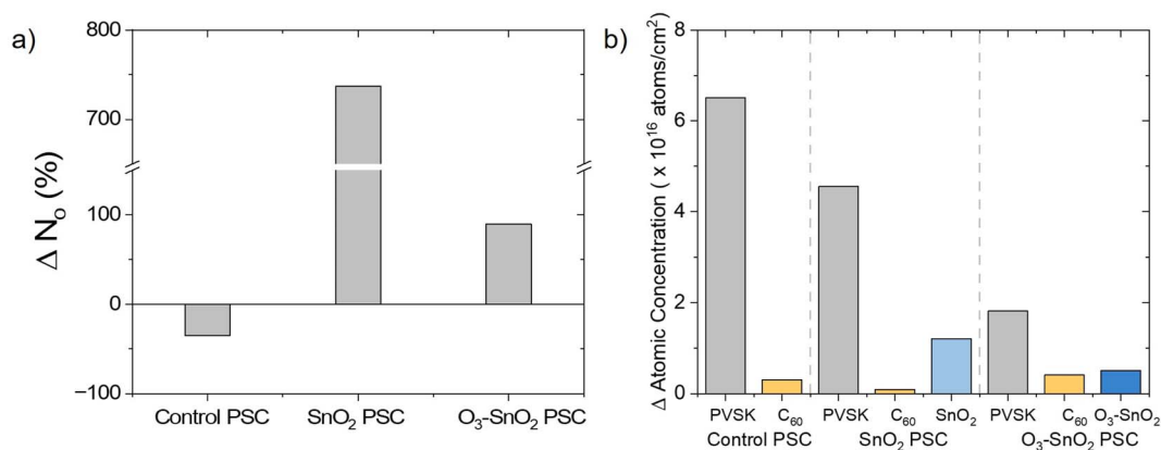
Fig. 2 Effectiveness of \text{SnO}_2 barrier layer in the prevention of Ag ion diffusion (a) percentage change in N_0 for control PSC, \text{SnO}_2 PSC, and \text{O}_3 - \text{SnO}_2 PSC with Ag top electrodes after exposure of the PSCs to 50 °C for 120 h. (b) Change in RBS atomic concentration of Ag after aging in the MHP layer and ETL for control PSC, along with barrier layer for \text{SnO}_2 PSC, and \text{O}_3 - \text{SnO}_2 PSC.
