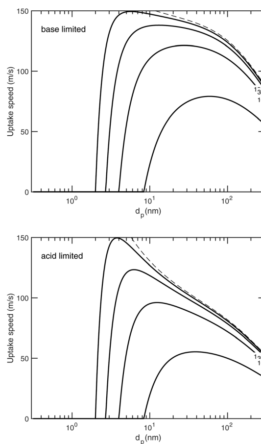
Fig. 17 Uptake speed ( \gamma_{i,p} S_{i,p}^+ L , black curves) vs. the diameter for flat-surface saturation ratios S^o = \{3, 10, 30, 100\} and d_{K10} = 2 \text{ nm} . The S^o = \infty limit is shown as a dashed curve. (Top) Base-limited ( \text{NH}_3 ) limited uptake assuming no van der Waals enhancement ( A = 0 \text{ joule} ). (Bottom) Acid-limited ( \text{HONO}_2 ) uptake with significant van der Waals enhancement ( A = 6 \times 10^{-20} \text{ joule} ). The collision speed (and thus growth rates) increases rapidly after activation, reaches a maximum and then declines again. The maximum is especially sharp when the van der Waals enhancement is large ( i.e. for acid limited conditions in the lower panel).
