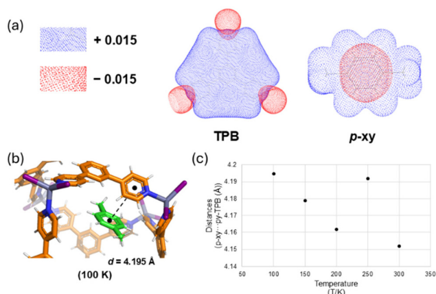
Fig. 4 (a) Plot of the MEPs of TPB and p -xy. (b) SC-XRD structure of 1 @100 K showing the distances among host and p -xy guest (guest A). (c) Graph with the evolution of the host-guest distances as a function of temperature.
