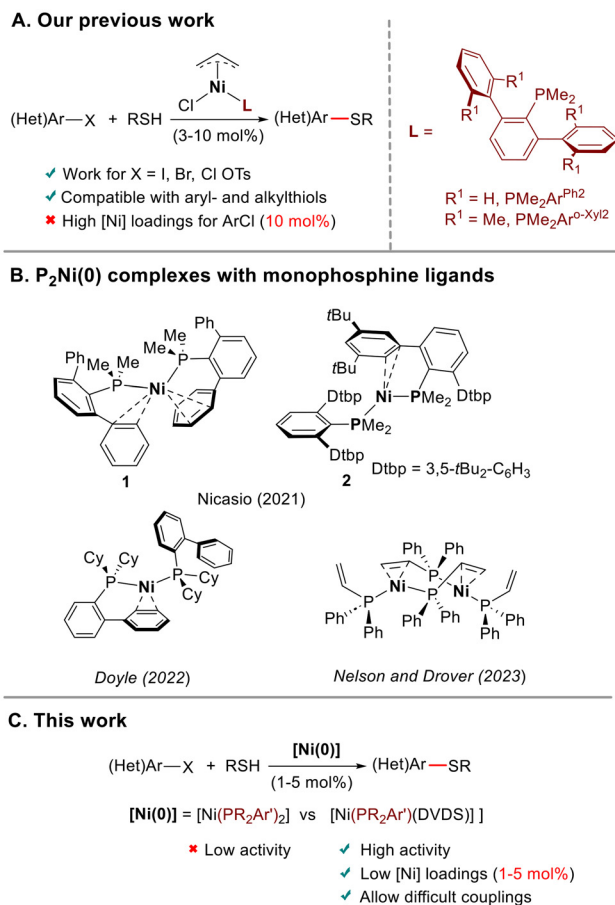
Scheme 1 (A) Our previous work on C–S cross-coupling using pre-formed Ni(II)-allyl precatalysts with terphenyl phosphine ligands. (B) \text{P}_2\text{Ni}(0) complexes with monophosphine ligands. (c) This work.
