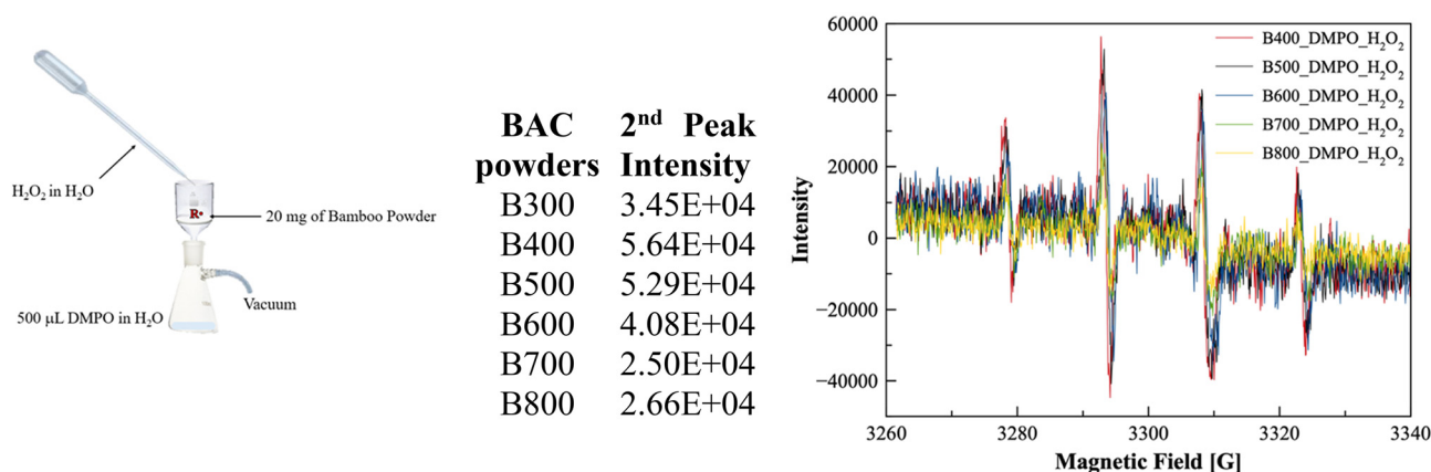
Fig. 10 Schematic illustration for generating stable paramagnetic \text{DMPO}^{\bullet}\text{-OH} species with a sintered glass filter connected to the vacuum system. 20 mg of BAC were weighed into the sintered glass filter, and 500 \mu\text{L} of a diluted \text{H}_2\text{O}_2 (2.68 mM) was percolated through it and dropped directly inside a flask containing 0.02 M of DMPO. EPR spectra of \text{DMPO}^{\bullet}\text{-OH} adducts in the final filtered solution (0.02 M of DMPO and 1.34 mM of \text{H}_2\text{O}_2 , in \text{H}_2\text{O} ) obtained from different BACs.
