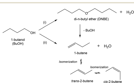
Scheme 1 Reaction pathways for 1-butanol dehydration: (i) intermolecular dehydration and (ii) intramolecular dehydration.
