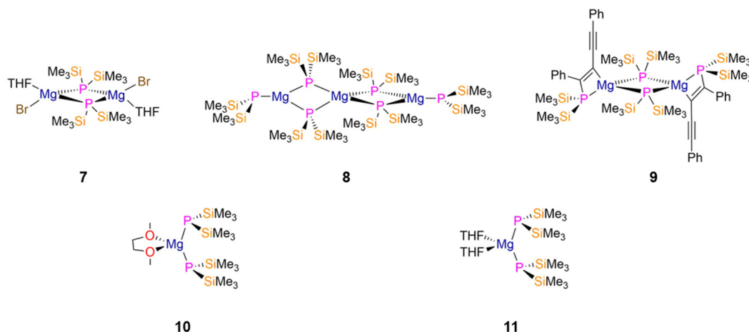
Fig. 3 Mg P'' complexes [\text{Mg}(\mu\text{-}P'')(\text{Br})(\text{THF})_2] ( 7 ), [\text{Mg}_3(\mu\text{-}P'')_4(P'')_2] ( 8 ), [\text{Mg}(P''\text{C}(\text{Ph})\text{C}(\text{C}_2\text{Ph}))_2(\mu\text{-}P'')]_2 ( 9 ), [\text{Mg}(P'')_2(\text{DME})] ( 10 ), [\text{Mg}(P'')_2(\text{THF})_2] ( 11 ).
