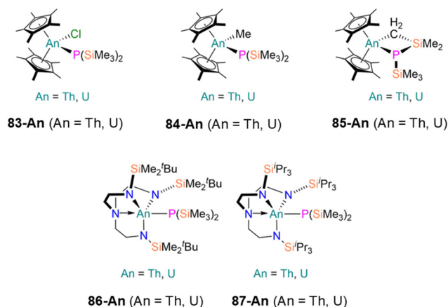
Fig. 24 An P'' complexes [\text{An}(P'')(\text{Cp}^*)_2(\text{Cl})] ( 83-An ; An = Th, U), [\text{An}(P'')(\text{Cp}^*)_2(\text{Me})] ( 84-An ; An = Th, U), [\text{An}\{\text{P}(\text{SiMe}_3)(\text{SiMe}_2\text{CH}_2)\}(\text{Cp}^*)_2] ( 85-An ; An = Th, U), [\text{An}(\text{Tren}^{\text{DMBS}})(P'')] ( 86-An ; An = Th, U), [\text{An}(\text{Tren}^{\text{TIPS}})(P'')] ( 87-An ; An = Th, U). \text{Tren}^{\text{DMBS}} = \{\text{N}(\text{CH}_2\text{CH}_2\text{NSiMe}_2^t\text{Bu})_3\} , \text{Tren}^{\text{TIPS}} = \{\text{N}(\text{CH}_2\text{CH}_2\text{NSi}^i\text{Pr}_3)_3\} .
