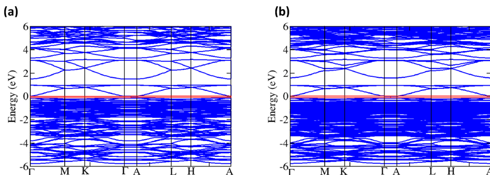
Fig. 3 Band structure for the (a) pure \text{In}_2\text{O}_3(001) surface and (b) Er-doped \text{In}_2\text{O}_3(001) surface.
