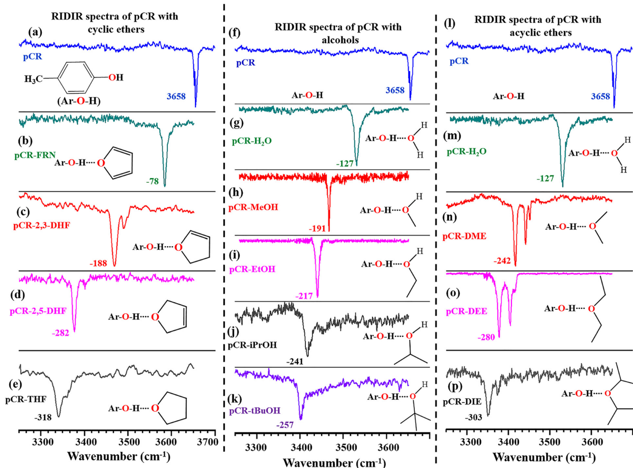
Fig. 1 Mass-selected vibrational spectra (RIDIR spectra) of Left Panel: H-bonded dimers of pCR with cyclic ethers, including (b) pCR-FRN, (c) pCR-2,3-DHF, (d) pCR-2,5-DHF, and (e) pCR-THF; Middle Panel: H-bonded dimers of pCR with alcohols, including (g)–(k) pCR with H 2 O, MeOH, EtOH, iPrOH, and tBuOH, respectively; Right Panel: H-bonded dimers of pCR with acyclic ethers, including (m)–(p) pCR with H 2 O, DME, DEE, and DIE, respectively. For comparison, the RIDIR spectrum of the pCR monomer is included at the top of each panel. The RIDIR spectra for the pCR-H 2 O, pCR-MeOH, pCR-EtOH, and pCR-DEE dimers have been previously reported in the literature; the experiments were reproduced here, yielding similar results. 53–55
