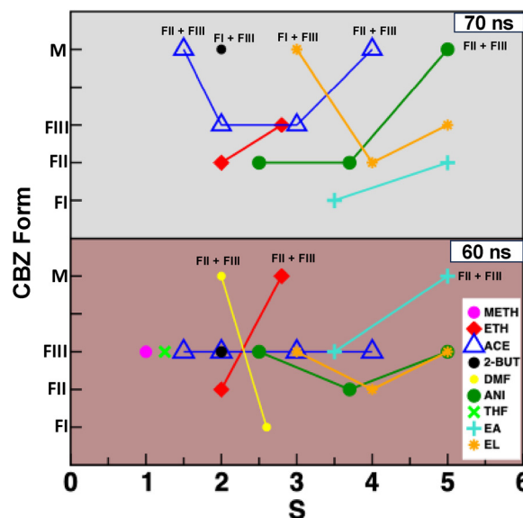
Fig. 7 CBZ dimers of FI-, FII-, and FIII-type as a function of supersaturation ( S ) in different solvents after t = 60 ns and 70 ns of NVT simulations; also shown are mixtures of different forms as M; lines are shown as a guide to show different supersaturation systems with the same solvent system.
