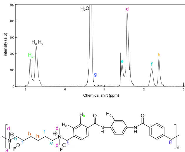
Fig. 2 Top: ^1H NMR of 6-F ionene solution at 8 g L^{-1} (0.014 mol L^{-1} , 300 MHz, D_2O solvent). Aromatic protons ( H_a , H_c and H_b ) appear at chemical shifts around 7–8 ppm, while aliphatic protons (d to h) appear in the range of 1.2–4.6 ppm. The strongest peak at 2.8 ppm (d) corresponds to methyl groups directly attached to the charged quaternary ammonium centers. Bottom: A schematic drawing of the ionene structure, indicating the different chemical environments for aromatic and aliphatic protons.
