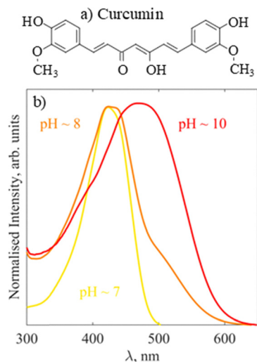
Fig. 1 (a) The structure of the enol tautomer of curcumin and (b) the UV/vis absorption spectrum of curcumin recorded under pH neutral (yellow, pH ~ 7), weakly basic (orange, pH ~ 8) and basic (red, pH ~ 10) conditions, where the solution is yellow, orange and red, respectively.
