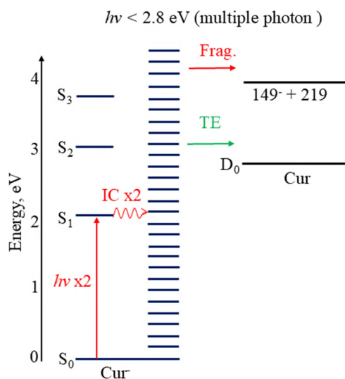
Fig. 6 The multiple-photon electron loss processes of Cur - observed in photoelectron imaging (Fig. 2). At h\nu < 2.8 eV, i.e. below the ADE of Cur - , photon cycling over the S_1 state is observed, which results in the formation of highly internally excited anions, which can fragment (red) or undergo thermionic emission (green). The processes are coloured to match the associated spectral features in Fig. 2.
