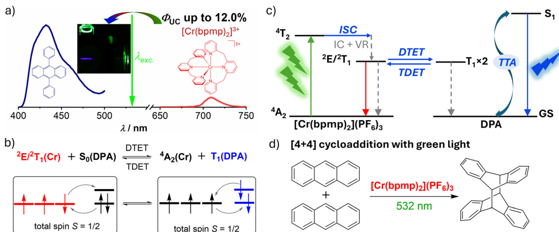
Fig. 2 Green-to-blue upconversion sensitized by a 3d^3 Cr(III) complex. (a) Photon upconversion luminescence spectrum of the [\text{Cr}(\text{bmpmp})_2](\text{PF}_6)_3/\text{DPA} pair under 532 nm laser excitation and their molecular structures. Inset: Image of the [\text{Cr}(\text{bmpmp})_2](\text{PF}_6)_3/\text{DPA} pair under green light irradiation. (b) Reaction scheme of the excited states of [\text{Cr}(\text{bmpmp})_2]^{3+} with the ground state DPA (DTET) and the reverse process TDET, accompanied with their relevant microstates. (c) Energy level diagram of sTTA-UC for the [\text{Cr}(\text{bmpmp})_2](\text{PF}_6)_3/\text{DPA} pair. ISC: intersystem crossing, IC: internal conversion, VR: vibrational relaxation, DTET: doublet–triplet energy transfer, TDET: triplet–doublet energy transfer, TTA: triplet–triplet annihilation. (d) [4+4] cycloaddition of anthracene catalyzed by [\text{Cr}(\text{bmpmp})_2](\text{PF}_6)_3 via sTTA-UC. 166 Reproduced under terms of the CC-BY license from ref. 166. Copyright 2022, Wiley-VCH.
