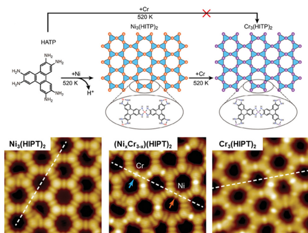
Fig. 14 Structural transformation by metal substitution from Ni_3(HITP)_2 through (Ni_xCr_{3-x})(HITP)_2 eventually to Cr_3(HITP)_2 frameworks on Au(111) in response to the addition of Cr atoms. Reproduced with permission. 170 Copyright 2023 Wiley-VCH GmbH.
